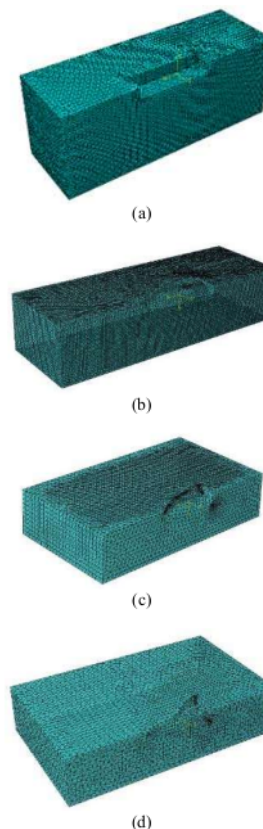
Figs. 8. Unstructured grid meshing model: (a) Conventional Model; (b) Fin-1 Model; (c) Fin-2 Model; (d) Fin-3 Model
