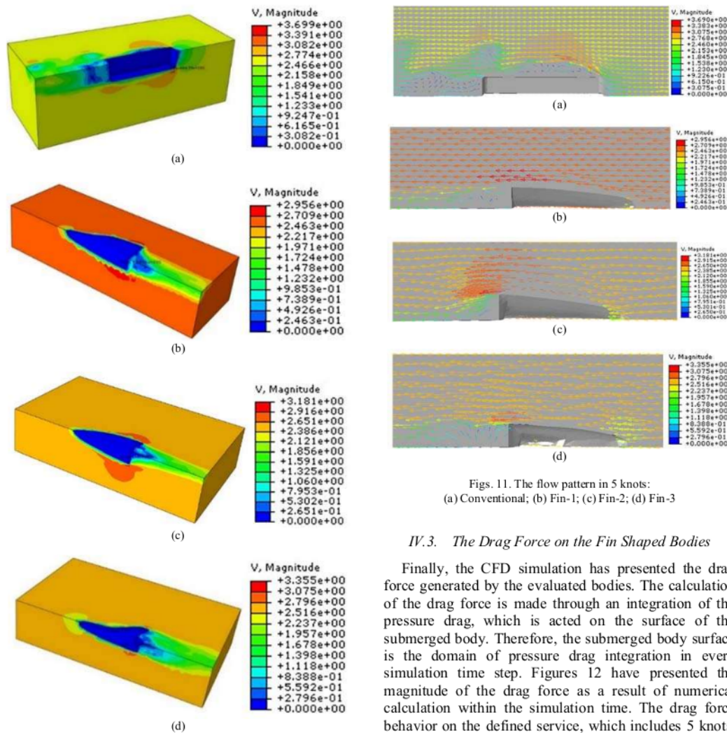
Figs. 10. The velocity distribution in 5 knot: (a) Conventional; (b) Fin-1; (c) Fin-2; (d) Fin-3
