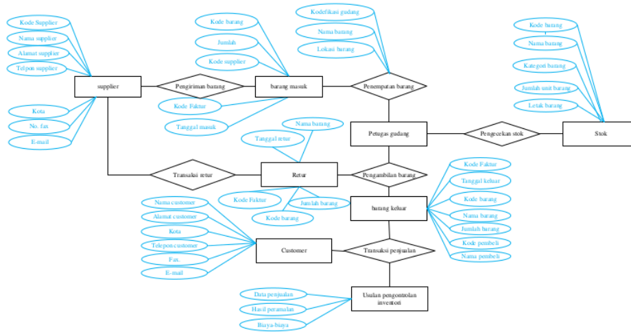
Gambar 12 Entity Relationship Diagram (ERD)
