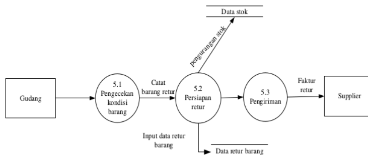
Gambar 10 DFD level 1 pengecekan stok
