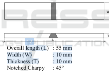
Figure 2: Impact test specimen (ASTM E23).
