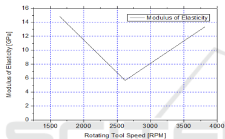
Figure 6: Modulus of elasticity of Aluminum 6061 at the defined rotating tool speed.
