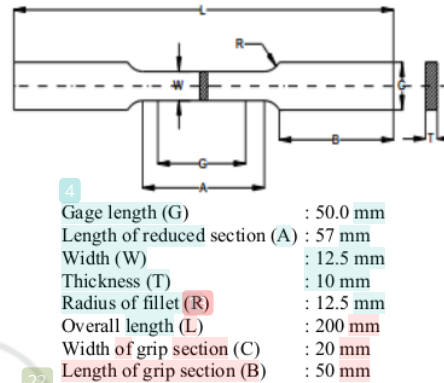
Figure 1: Tensile test specimen (ASTM E8/E8M-09).
