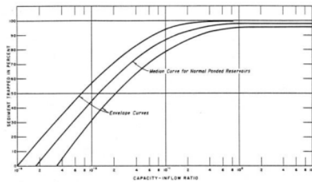
Gambar 1. Kurva trap efficiency [5]
