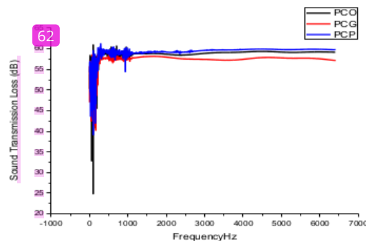
Gambar 2.11. Hasil Uji Sound Transmission Loss
