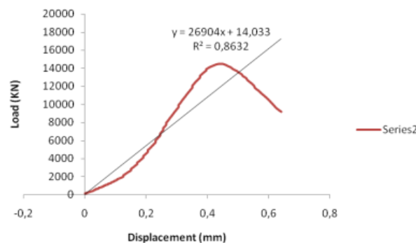
Gambar 5.1. Modulus Elastisitas Beton Foamed
