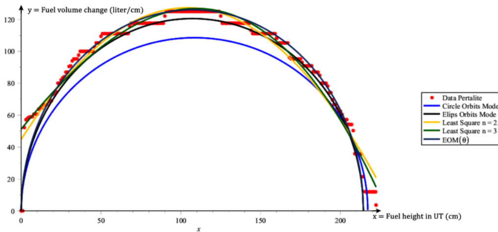
Figure 7. Comparison Graph of Approximation Method Results
