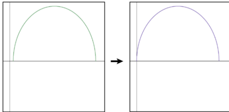
Figure 4. Visualization of Steps in (6) to (7)
