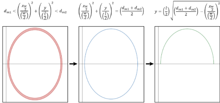
Figure 3. Visualization Steps in (6)
