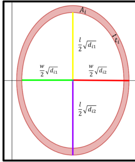
Figure 1. Set Visualization A_i (2)
