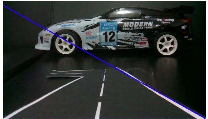
Fig. 10. Resulted line detection.
