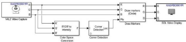
Fig. 7. Block diagram of corner detection in Simulink block diagram.
