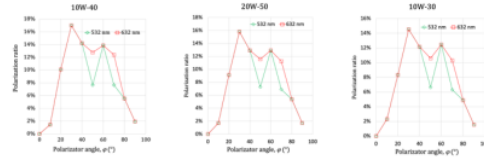
Fig.6: Natural polarization ratio at wavelengths of 532 m and 632 nm for the three samples. There is a birefringent phenomenon at angles \varphi = 50^\circ and \varphi = 70^\circ in all samples. The results of a preliminary study using 20W-50 [18] also showed the same phenomenon.
