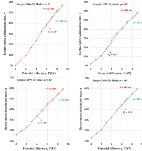
Fig.10: Electro-optical polarization ratio for 20W-50 oil at 532 nm and 632 nm wavelengths. In the \varphi = 0^\circ, 30^\circ, 60^\circ , and 90^\circ modes after critical V_k , the optical axis is split into two.
