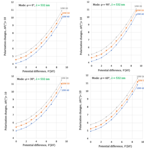
Fig.7: Electro-optical polarization change for three oils at a wavelength of 532 mn.
