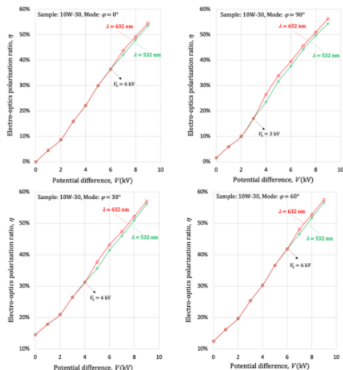
Fig.11: Electro-optical polarization ratio for 10W-30 oil at 532 nm and 632 nm wavelengths. In the mode \varphi = 0^\circ , 30^\circ , 60^\circ , and 90^\circ after the critical voltage V_k , the optical axis is split into two.
