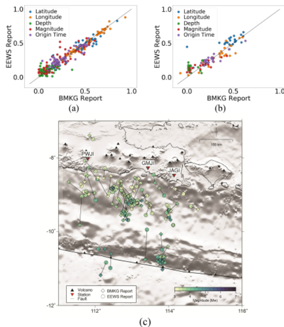
Fig. 4. Distribution of an earthquakes' parameter reported by the BMKG and proposed EEWS (a) 62 validation data, (b) 26 data in 2019, and (c) epicenters of earthquakes.
