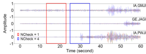
Fig. 3. Example of the real-time PTWP with a validation data of 2017.
