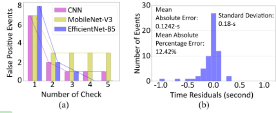
Fig. 2. (a) Comparison of the number of N in the NCheck algorithm from N1 to N5 and (b) optimal result of N4 is in the EfficientNet-B5 model with the best validation learning scheme.
