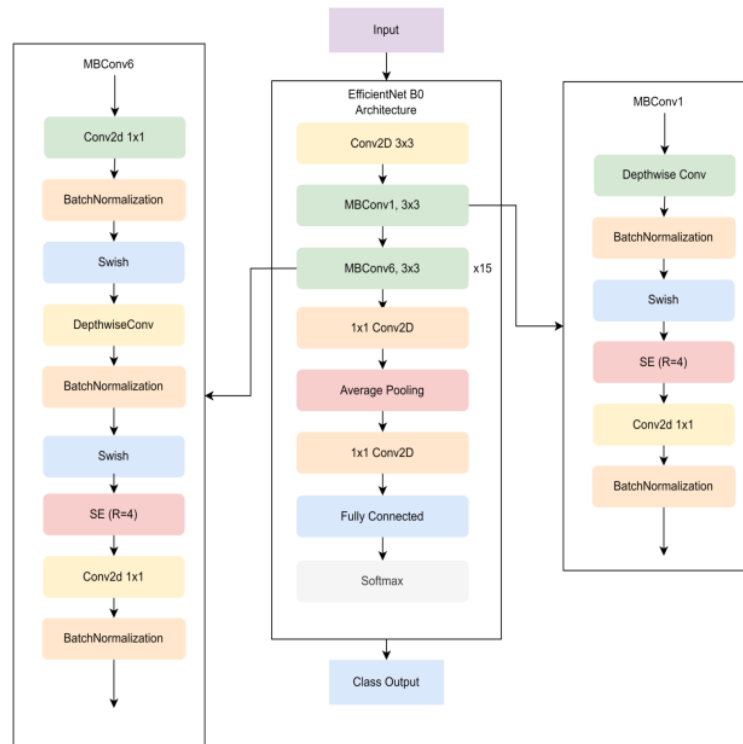
Figure 7. The EfficientNet B0 Network.
