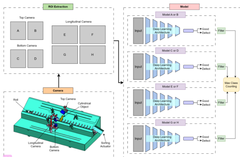
Figure 1. The framework of the proposed method.
