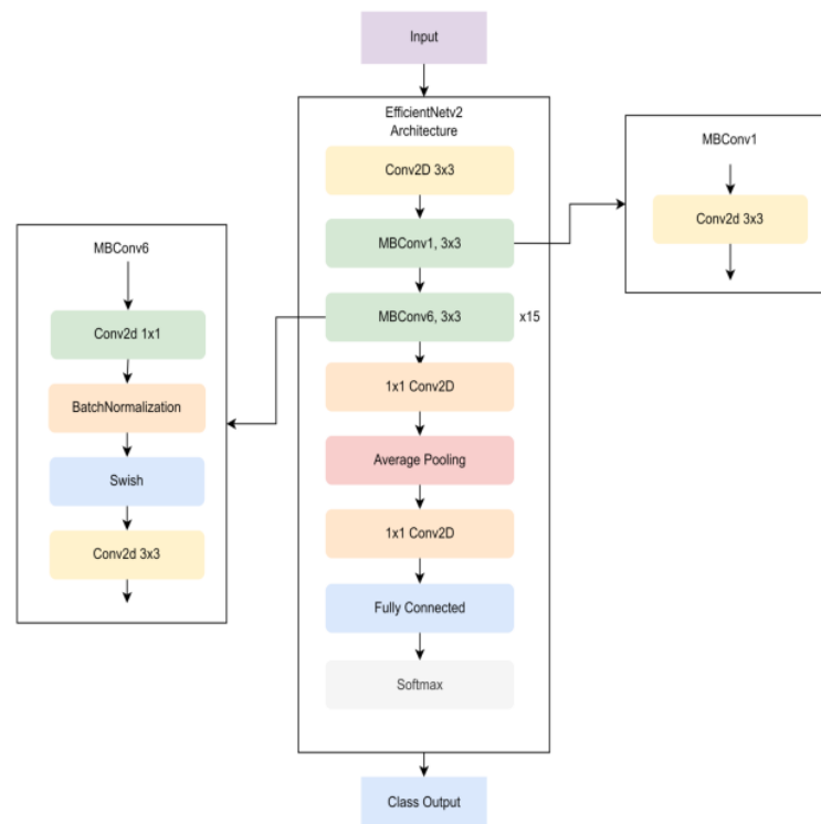
Figure 8. The EfficientNet v2 Network.
