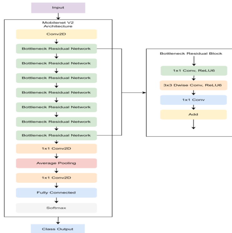
Figure 6. The MobileNet v2 Network.
