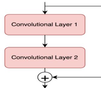
Figure 4. Residual Network.
