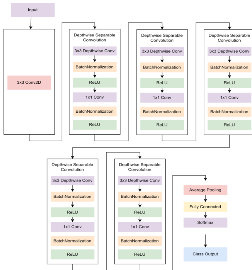
Figure 5. The MobileNet v1 Network.
