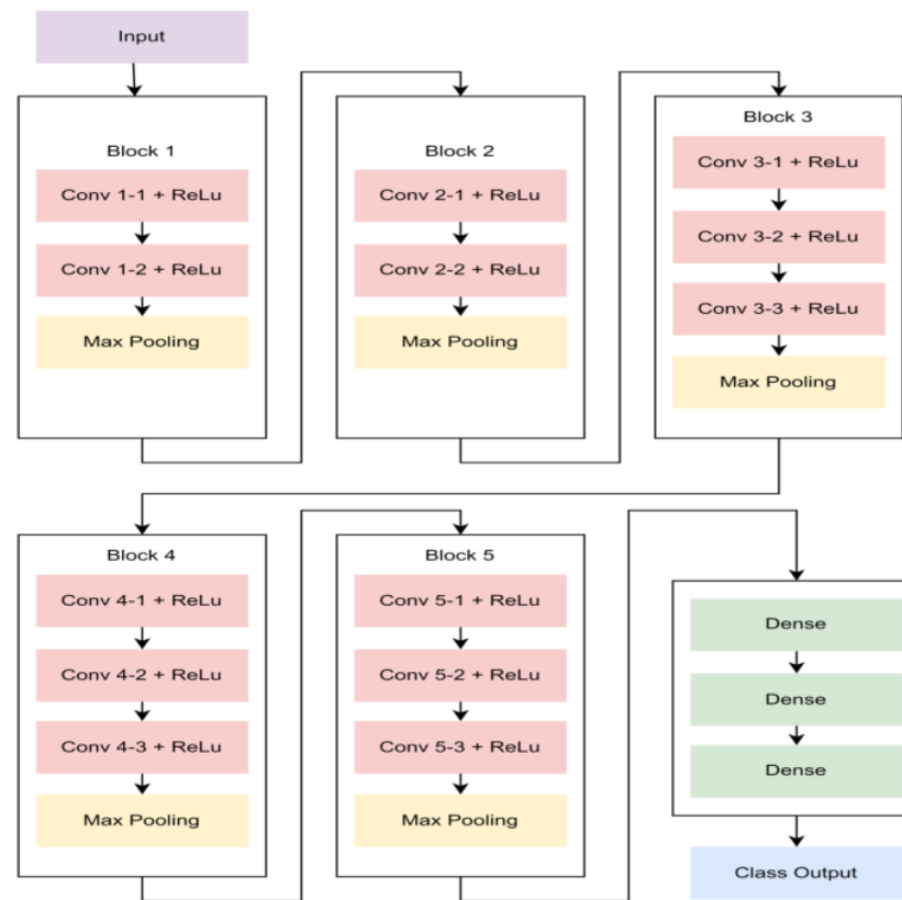
Figure 3. The VGG16 Network
