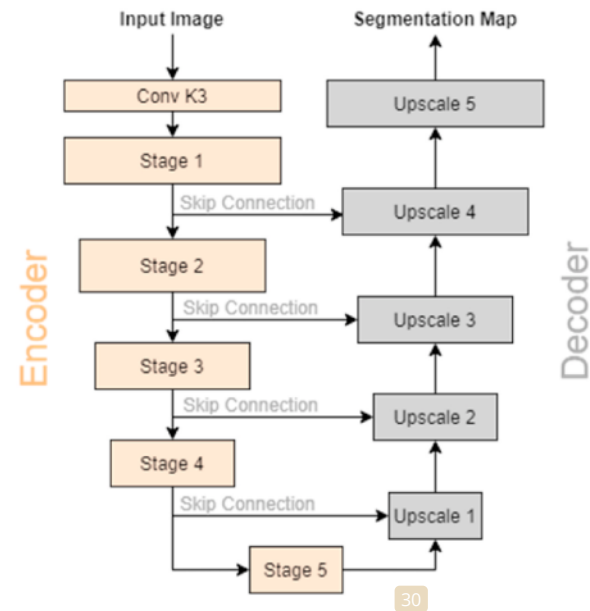
Fig. 3. Proposed decoupled encoder and decoder modules in an end-to-end semantic segmentation architecture.
