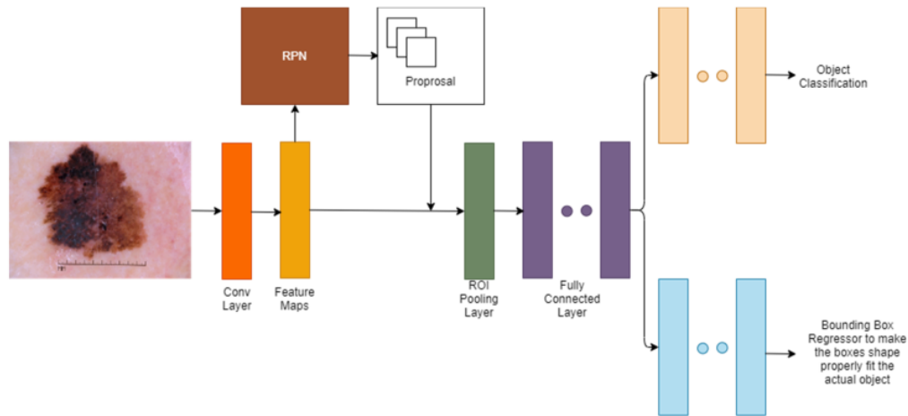
Fig. 4. Faster R-CNN architecture model
