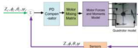
Gambar 4. Model PD nonlinear
