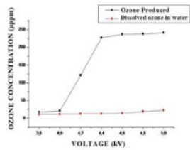
Figure 9. Comparison value concentration of Ozone produced and dissolved Ozone in water with contant time of 5 minutes for oxygen flow rate of 1.5 liters/minute
