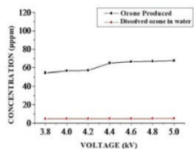
Figure 10. Comparison value concentration of Ozone produced and dissolved Ozone in water with contant time of 5 minutes for dry air flow rate of 1.5 liters/minute
