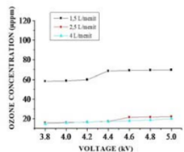
Figure 5. Concentration of ozone as function voltage with time constant of 4 minutes and rate flow of dry air of 1.5 liters/minute, 2.5 liters/minute 4.0 liters/minute
