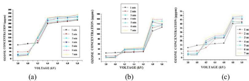
Figure 2: Ozone concentration as function of voltage with certain time of constant with flow rate of oxygen (a). 0.5 L/minutes, (b). 1.5 L/minutes, and (c). 2.5 L/minutes
