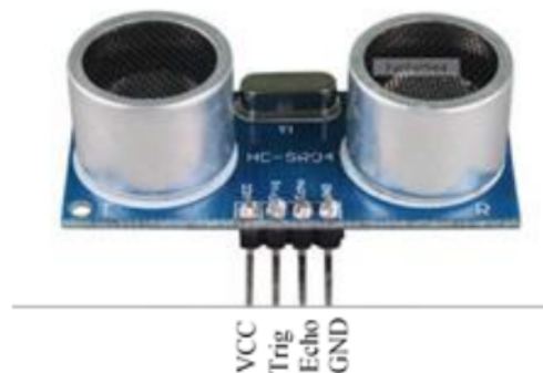
Gambar 3. Modul sensor ultrasonik HC-SR04
