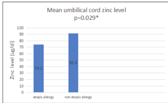
Figure 2. Zinc level between two groups
