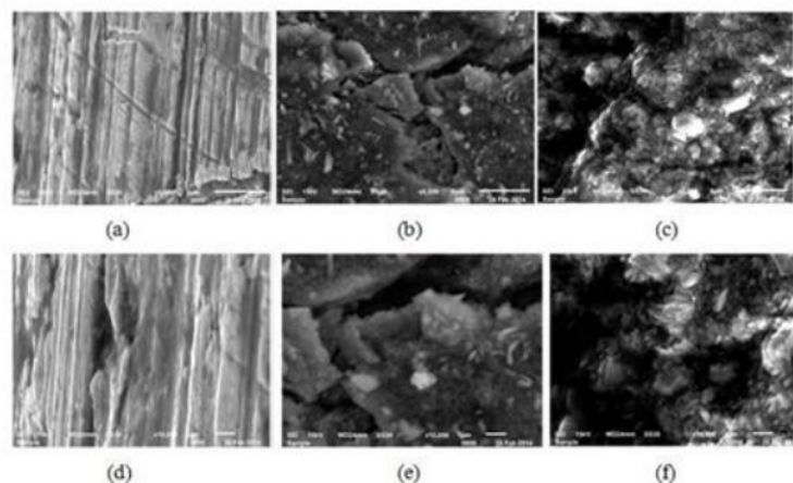
Figure 12. SEM images of the surface morphology of the Cu electrodes with diameter of 0.52 mm, top 5000 \times , 10000 \times bottom. (a & d) before use, (b & e) after use, (c & f) after use and washed.
