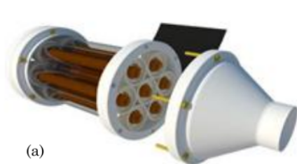
Figure 2. Integrated ozone generator with seven DBD reactors (a) Design (b) Realization
