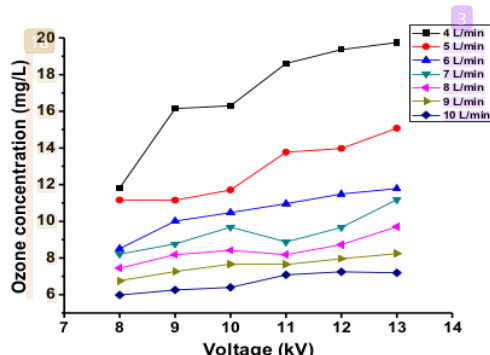
Figure 4. Ozone concentration as function of applied voltage for air flow rate variations.
