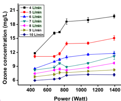
Figure 6. Ozone concentration as a function of input power.
