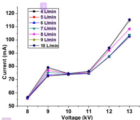
Figure 3. Current as function of voltage, for integrated reactor, for all variants air flow rate.
