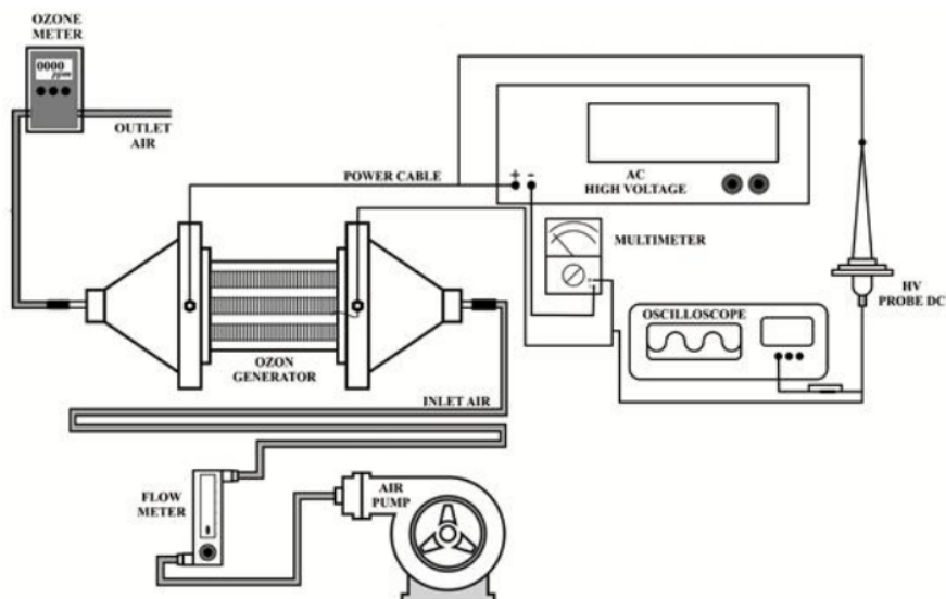
Figure 1. Experimental set up for an integrated ozone generator
