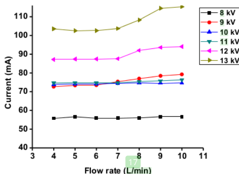
Figure 5. Electric current as a function of air flow rate for some voltage variation.
