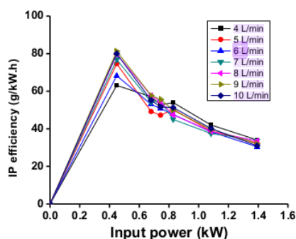
Figure 8. Input Power Efficiency as a function of input power at flow rates of 4-10 L/min with interval of 1 L/min
