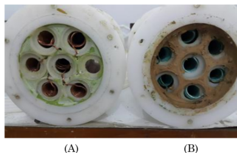
Figure 11. Photographs of reactor with electrodes in the form of spiral coil copper before (A) and after used (B)
