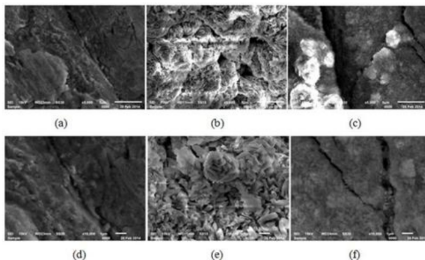
Figure 13. SEM image of the surface morphology of the Cu electrode with diameter of 1.12 mm, top 5000 \times , 10000 \times bottom (a & d) before use, (b & e) after use, (c & f) after use and washed
