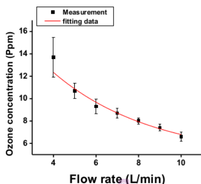
Figure 10. The average ozone concentration as a function of air flow rate
