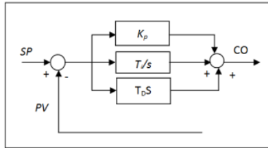
Gambar 1. Diagram blok kendali PID ideal.
