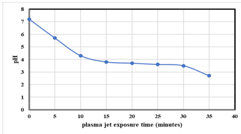
Fig. 2 Graph of pH as functions of plasma jet exposure time
