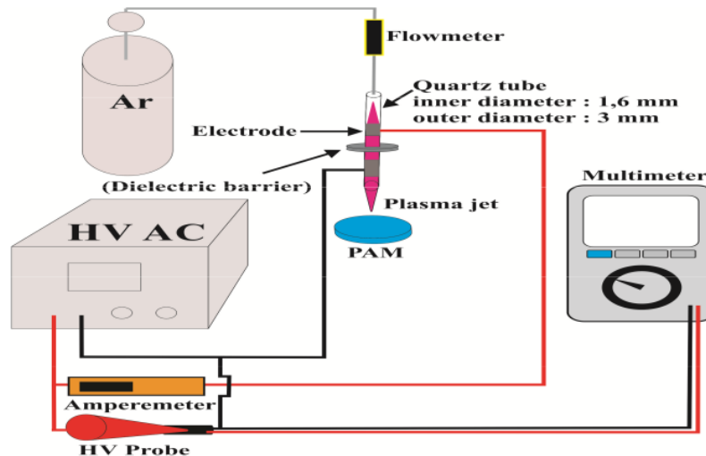
Fig. 1 Schematic of research equipment set-up
