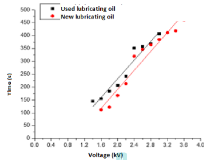
Fig 9:- Graph of the difference in the effect of voltage on the union time at the distance between the electrodes (d) = 12 mm
