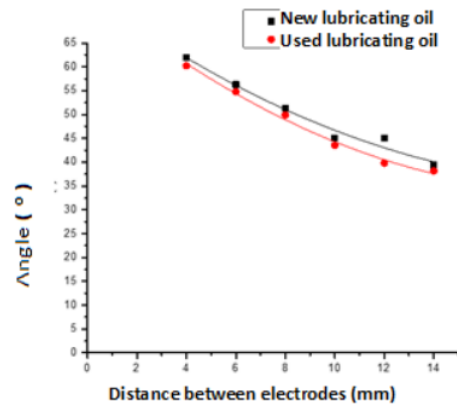
Fig 7:- Comparative graph of the relationship between the ion wind direction angle as function of the distance between the electrodes for new and used lubricant oil at a voltage (V)=1.6 kV
