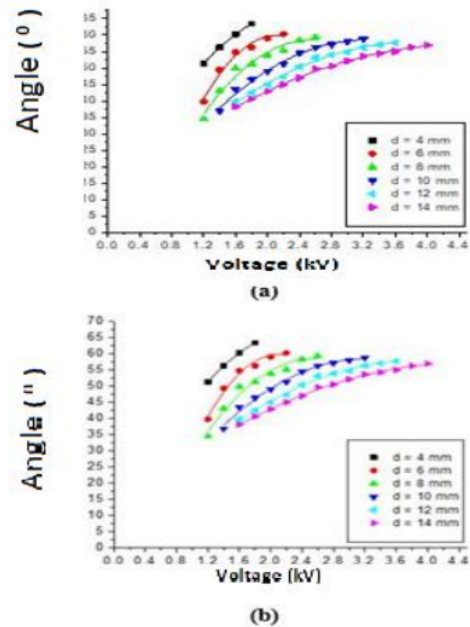
Fig 6:- (a) Used lubricating oil (b) new lubricating oil. Effect of voltage on ion wind angle
