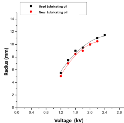
Fig 4:- Radius of circle deformation of used and new lubricant oil as function of applied voltage
