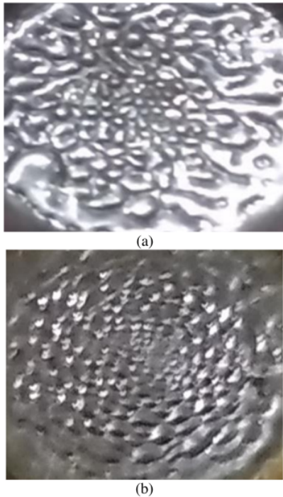
Fig 5:- (a) New lubricating oil (b) used lubricating oil EHD Flow phenomena
