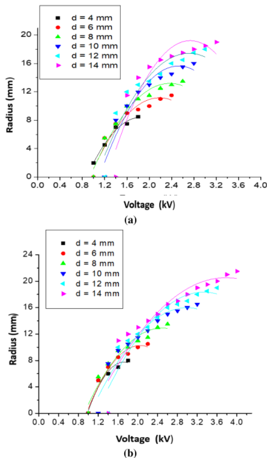
Fig 3:- (a) Used lubricating oil (b) new lubricating oil. The deformation's radius of lubricant oil in EHD phenomenon as function of applied voltage
