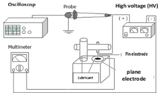
Fig 1:- Schematic of the research circuit
