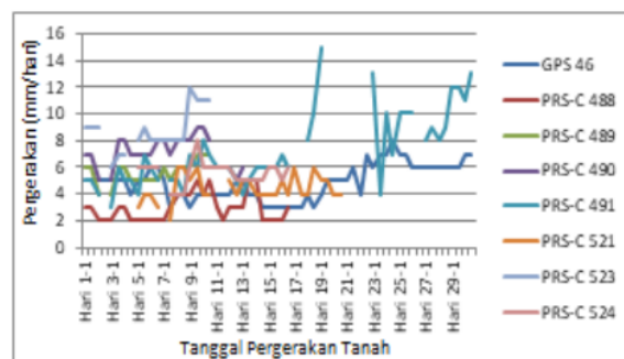
Gambar 1. Grafik Monitoring Pergerakan Lereng September 2020.
