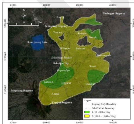
Figure 7. Aquifer storage.
