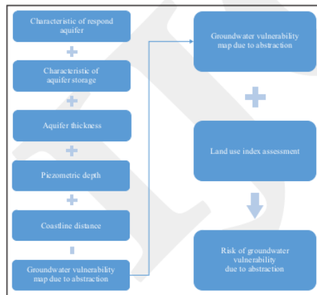
Figure 5. Spatial analysis processes to define the risk of groundwater vulnerability to abstraction.
