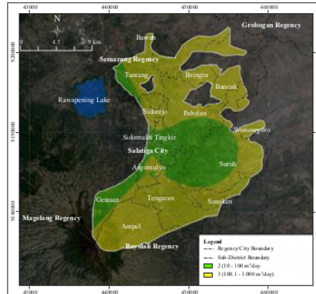
Figure 9. Piezometric depths.
