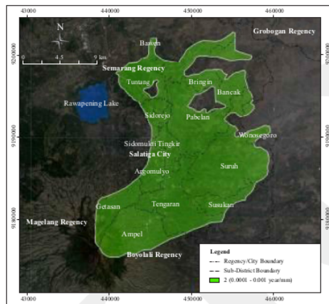
Figure 6. Respond aquifer.
