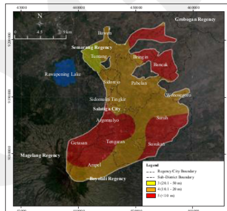
Figure 8. Aquifer thickness.
