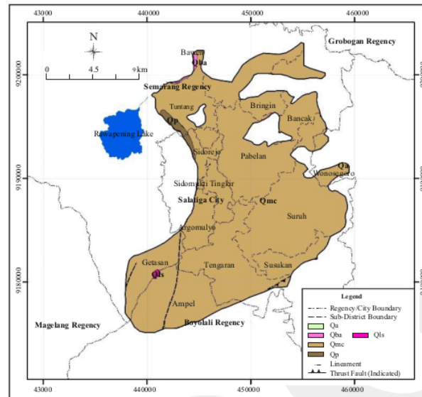
Figure 2. Regional geological map of Salatiga Groundwater Basin.
