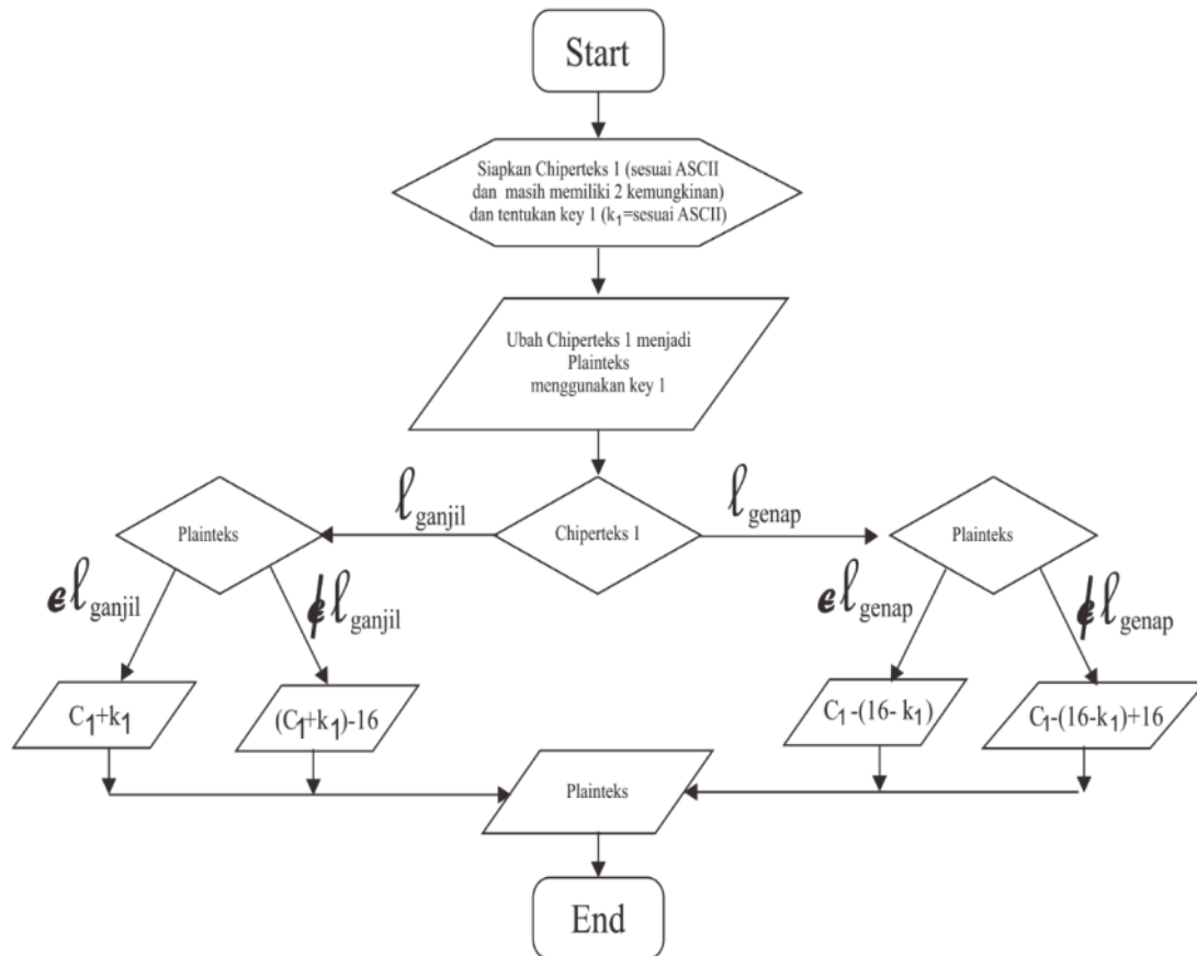
Figure 6. Cipherteks 1 to Plainteks
