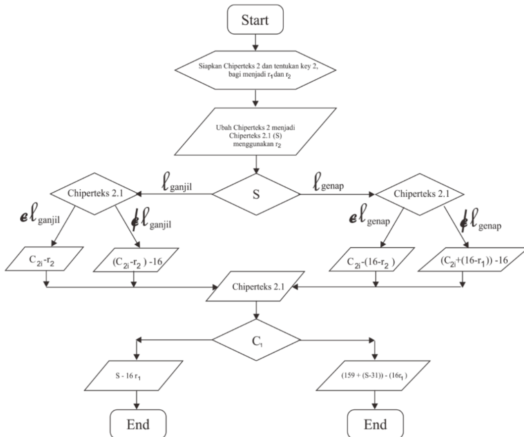
Figure 5. Chipertext 2 to Cipherteks 1
