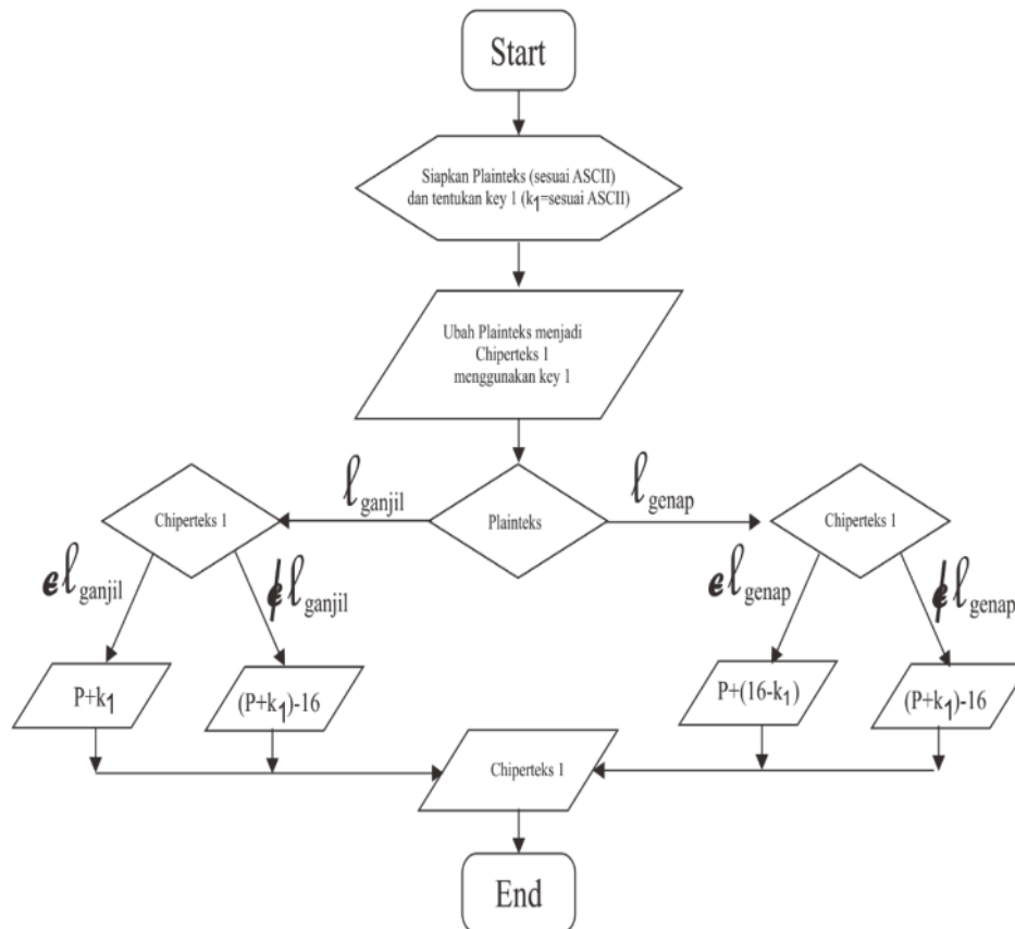
Figure 3. Plaintext to Cipherteks 1
