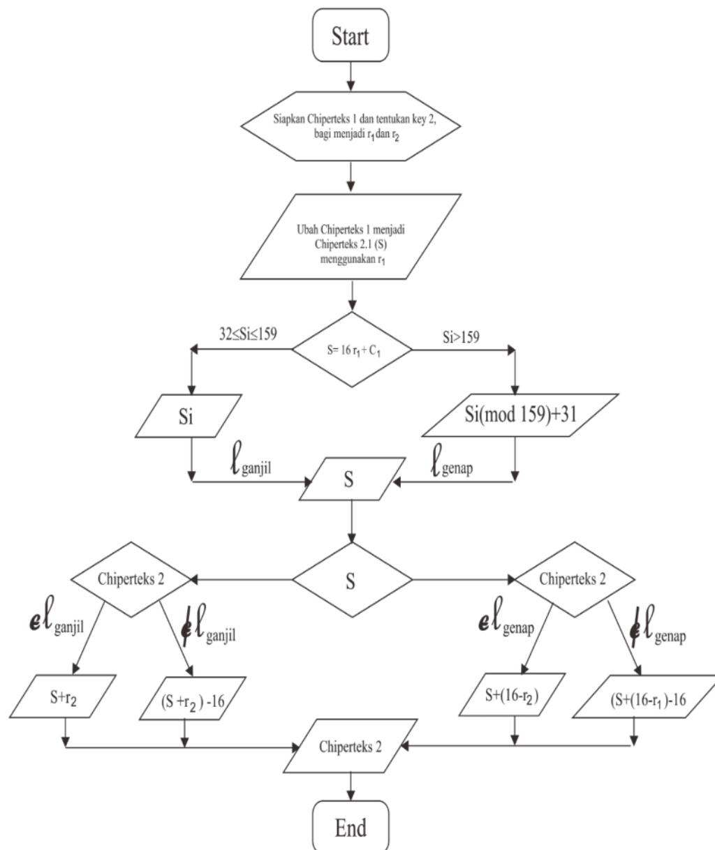
Figure 4, Chipertext 1 to Cipherteks 2
