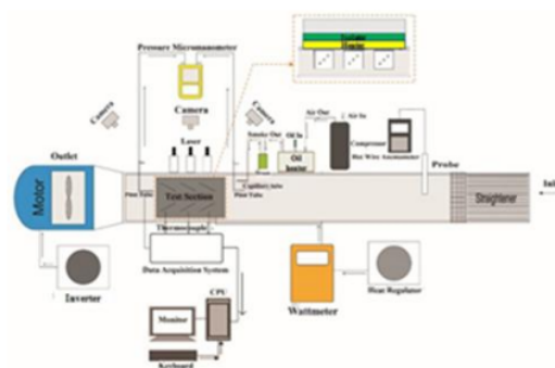
Figure 1. Experimental set-up
