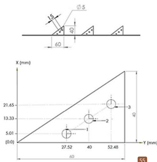
Figure 2. Detail geometry of perforated concave and plain delta winglet vortex generators
