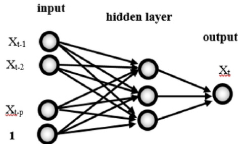
Figure 1. Neural network architecture for time series prediction
