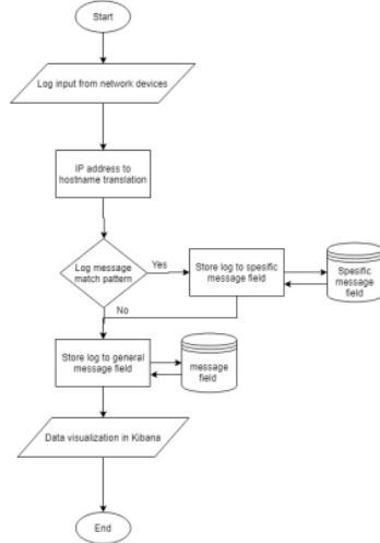
Figure 3. Flow chart of Log Management System
