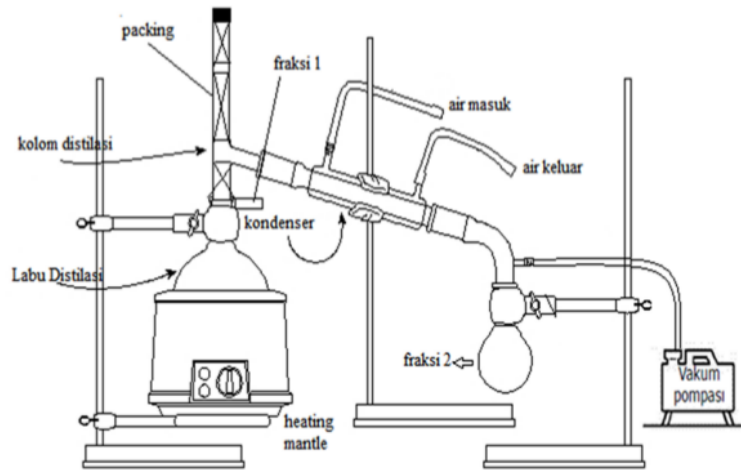
Figure 2. Vacuum Distillation equipment
