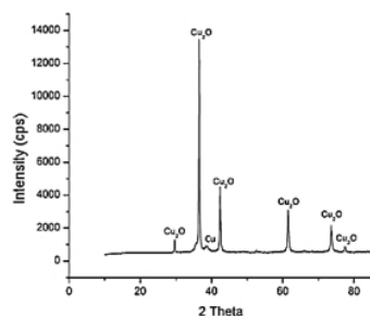
Figure 5. XRD results of \text{Cu}_2\text{O} powder from synthesis with a Cu: citrate mole ratio of 1: 2.
