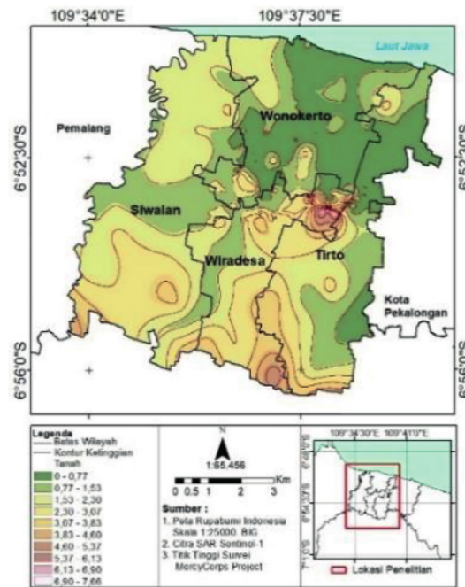
Figure 4. Ground elevation map generates by DEM process
