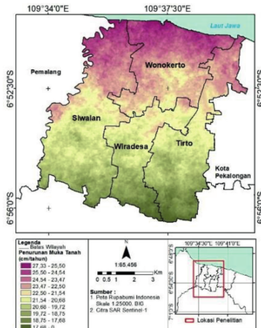
Figure 3. Land subsidence year 2017–2020
