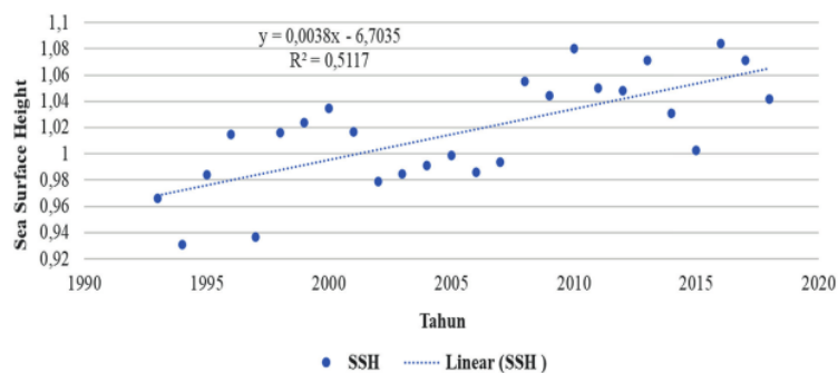
Figure 2. Graphic of sea level anomaly
