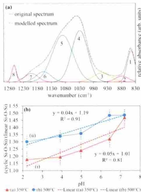
Fig. 4. (a) Deconvoluted FTIR spectra, spectra 1 to 8 are derived spectra obtained from the deconvolution of the original spectra, (b) DMDMS-TEOS (cyclic Si-O-Si/linear Si-O-Si) ratio of silica xerogel calcined at (i) 350 °C and (ii) 500 °C as a function of pH. The dotted lines indicate a linear trendline.
