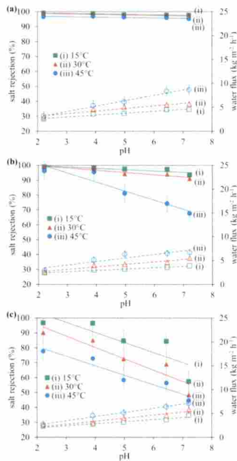
Fig. 10. Salt rejection (filled bullet) and water flux (empty bullet) of DMDMS-TEOS silica membranes at NaCl concentrations of (a) 0.3 wt.% (b) 1 wt.% (c) 3.5 wt.%.
