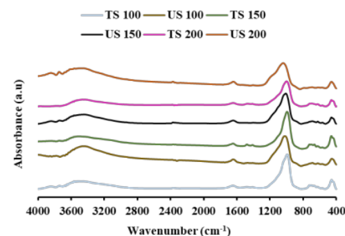
Figure 4. FTIR spectra of silica-rich sodalite zeolite with and without ultrasound treatment
