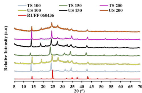
Figure 2. Diffractogram of silica-rich sodalite zeolite with and without ultrasound treatment and RUFF 060436
