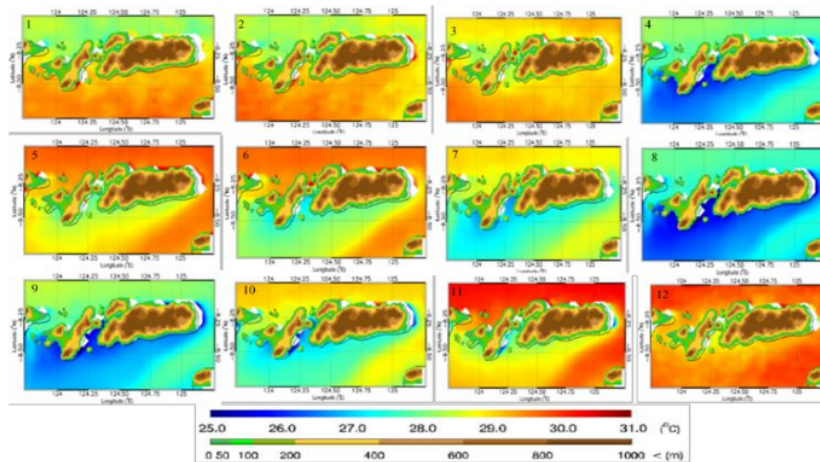
Figure 9. Monthly (1-12) average of sea surface temperature 2020.
