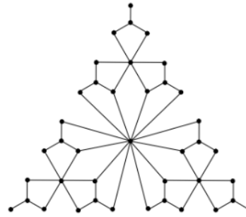
Gambar 1b. Graf SS_4
