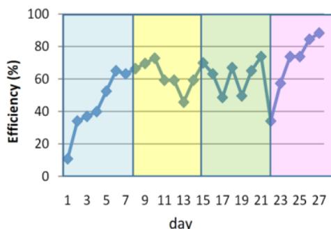
Fig.2. Chart of efficiency of BOD concentration decreasing on Anaerobic condition.
