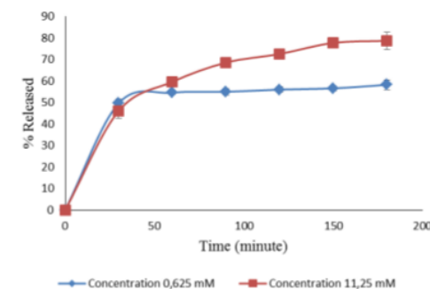
Figure 5. Release profile encapsulation rutin on PBS medium at pH 7,4
