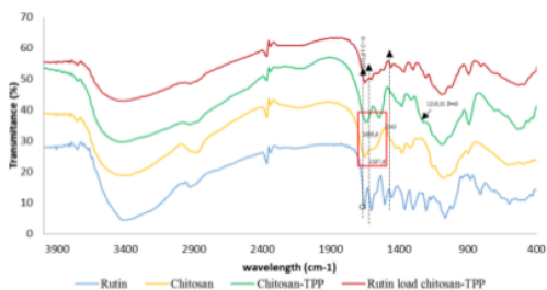
Figure 6. Spectra of rutin, CS, CS-TPP and rutin load CS-TPP microparticle using FTIR
