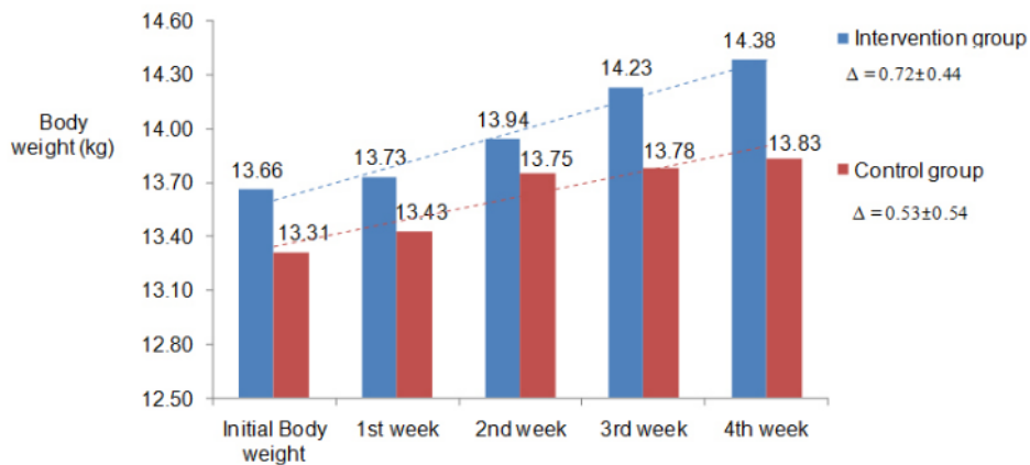
Fig. 3: Histogram of the average of W/A of under five subjects before and after 30 days study. There was significant increase of body weight in each group after 30 days study (Wilcoxon test with p = 0.001) in which the increase in intervention group was higher (0.72 kg) compared to control group (0.53 kg). Increase B/A between intervention and control group were not significant (Mann Whitney test with p = 0.830)
