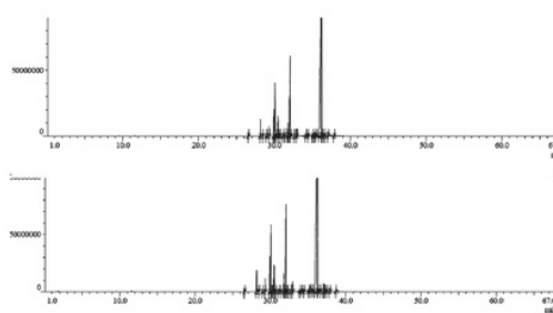
Fig. 2. Chromatogram of improving patchouli plant (top) and Batang local patchouli plant.
