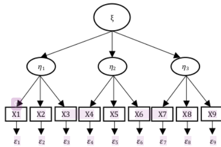
Gambar 3 Diagram Second Order CFA
