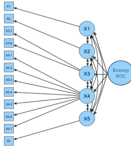
Gambar 4 Diagram CFA Model Akhir
