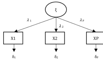
Gambar 2 Diagram First Order CFA
