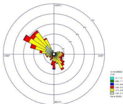
Figure 3. Prevailing wind at Semarang city throughout the year.
