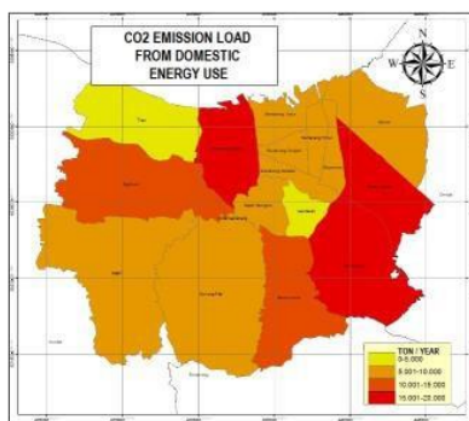
Figure 2. CO 2 emission load from domestic sector.
