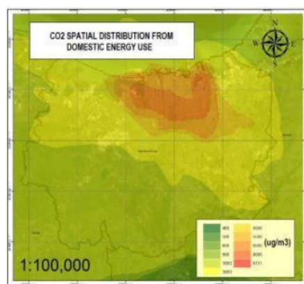
Figure 4. CO 2 emission dispersion from domestic sector.
