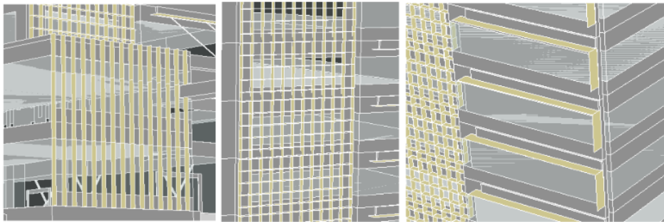
Figure 4. Detail on the application of the vertical combination: vertical combination (left), eggrate (center), L shape (right).
