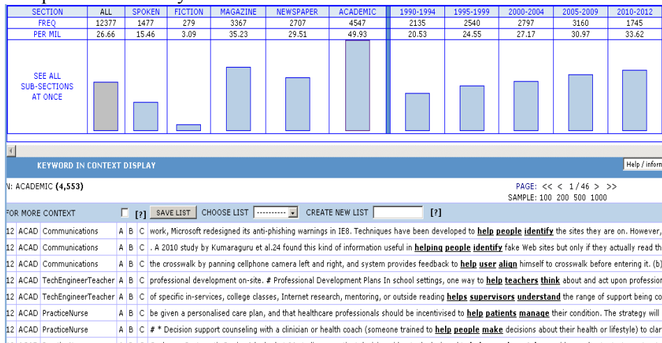
Figure 17: The Concordance of <help><N><Vinf>
