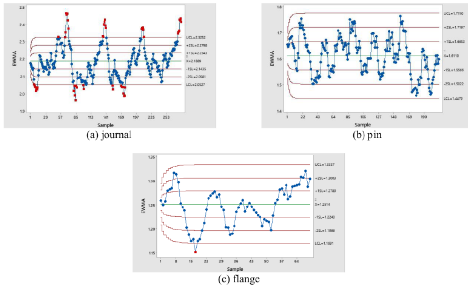
Figure 7. EWMA control chart design
