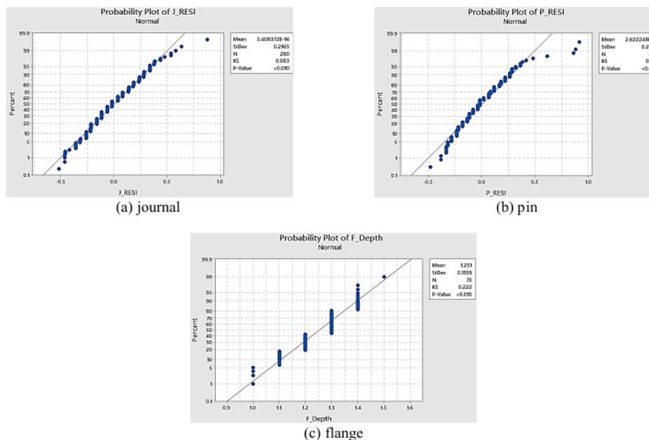
Figure 5. Normality test result
