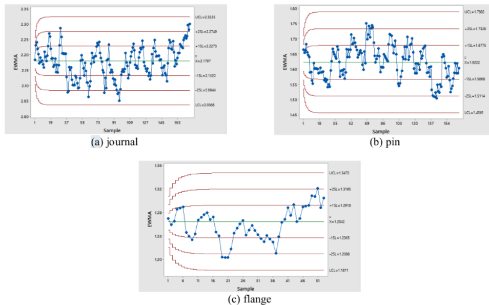
Figure 8. EWMA control chart design
