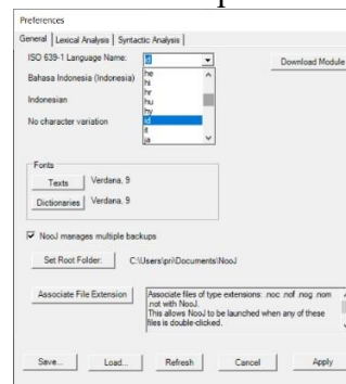
Figure 2 SANTI-morf Activation via NooJ's Preferences
