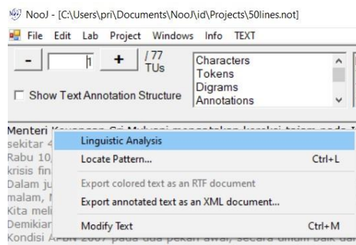
Figure 7. Corpus annotation
