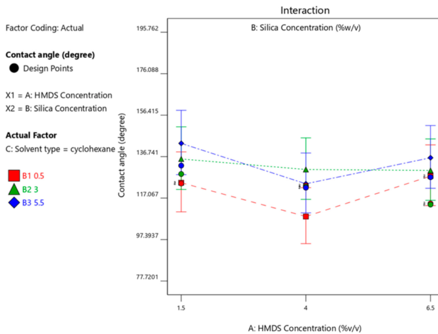
Figure 6. Contact angle response interaction between HMDS and silica concentration with cyclohexane solvent.
