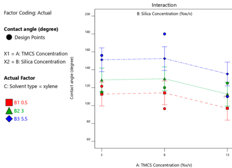
Figure 14. Contact angle upon interaction between TMCS and silica concentration with xylene solvent.
