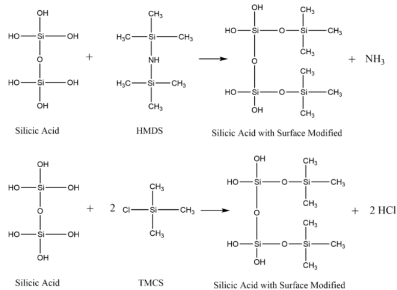
Figure 11. Formation reaction using HMDS and TMCS [28].
