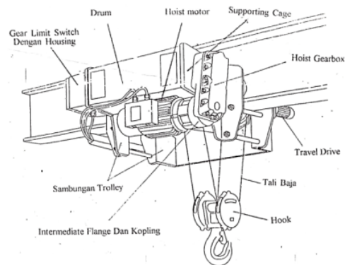
Gambar 1. Hoist Crane [4]
