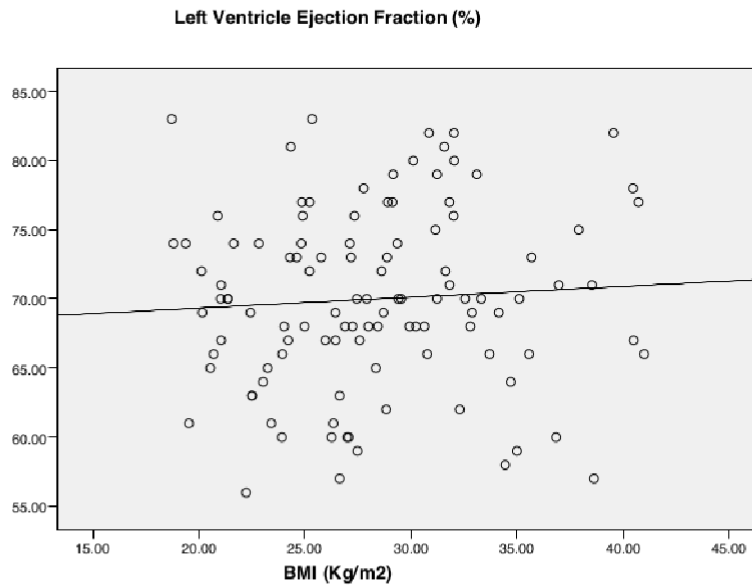
3 Fig. 2. Correlation between BMI and LVEF (r=0,06;p=0,49)
