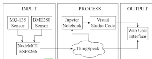
Figure 1. Block diagram of system
