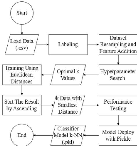
Figure 4. Dataset processing flow diagram using k-NN algorithm
