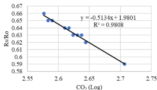
Figure 5. Graph of relationship between CO_2 concentration and resistance ratio R_s/R_0
