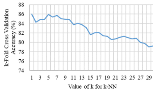
Figure 6. Optimal k values of k-NN obtained through k-fold cross validation
