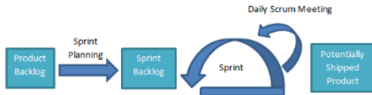
Figure 1: Scrum Process
