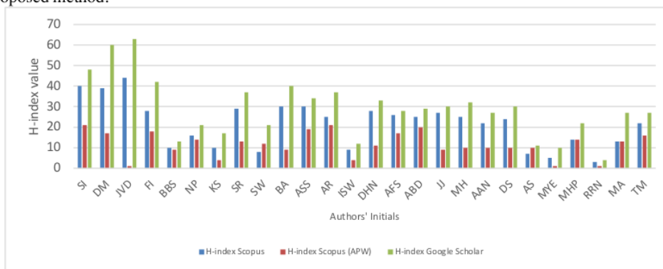
Figure 1. Distribution of H-index values based on Sinta Index Rank.
