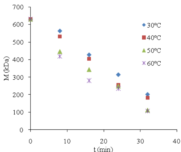
Figure 1. Effect of temperature on the number-average molecular weight of \kappa -carrageenan upon ultrasound-assisted hydrolysis at initial pH 6
